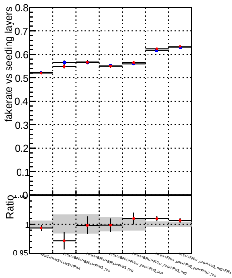
Fake rate vs. \chi^2 vs seeding layers
