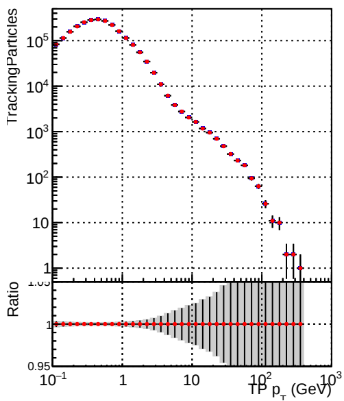
—•— DQM_CKF_TTbase —•— DQM_CKF_TT_retrainOldFiles125_v2_prelimWP2_epoch4
