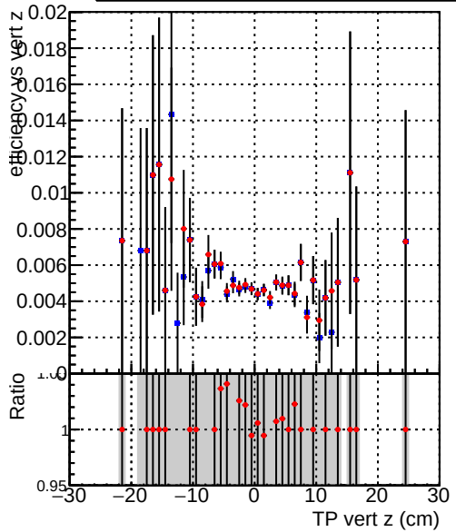
Efficiency vs TP vert z —●— DQM_CKF_TTbase —●— DQM_CKF_TT_retrainOldFiles125_v2_prelimWP2_epoch4
