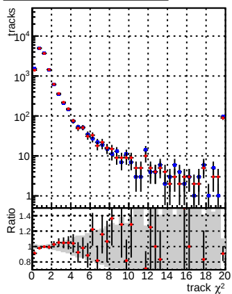
N of reco track vs. \chi^2 for DQM_CKF_TTbase vs DQM_CKF_TT_retrainOldFiles125_v2_prelimWP2_epoch4
