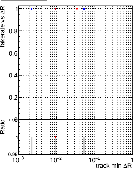
Fake rate vs ΔR(track, jet) Legend: DQM_CKF_TTbase (blue squares) DQM_CKF_TT_retrainOldFiles125_v2_prelimWP2_epoch4 (red circles)
