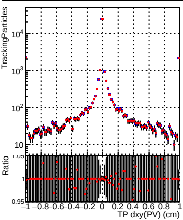
N of sim DQM_CKF_TT_retrainOldFiles125_v2_prelimWP2_epoch4
