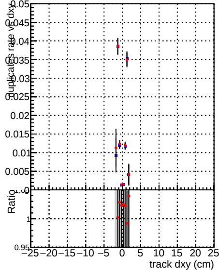
—■— DQM_CKF_TTbase —●— DQM_CKF_TT_retrainOldFiles125_v2_prelimWP2_epoch4
