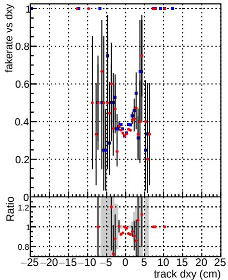
—■— DQM_CKF_TTbase —●— DQM_CKF_TT_retrainOldFiles125_v2_prelimWP2_epoch4
