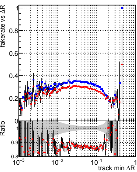
Legend: DQM_CKF_TTbase (blue line with dots), DQM_CKF_TT_retrainOldFiles125_v2_prelimWP2_epoch4 (red line with dots)
