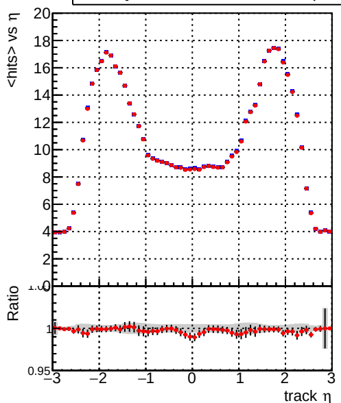
— DQM_CKF_TTbase — DQM_CKF_TT_retrainOldFiles125_v2_prelimWP2_epoch4 mean hits vs \eta
