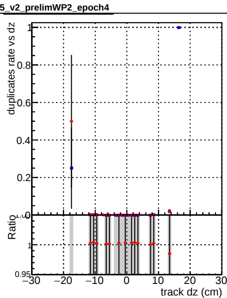
—●— DQM_CKF_TTbase —●— DQM_CKF_TT_retrainOldFiles125_v2_prelimWP2_epoch4
