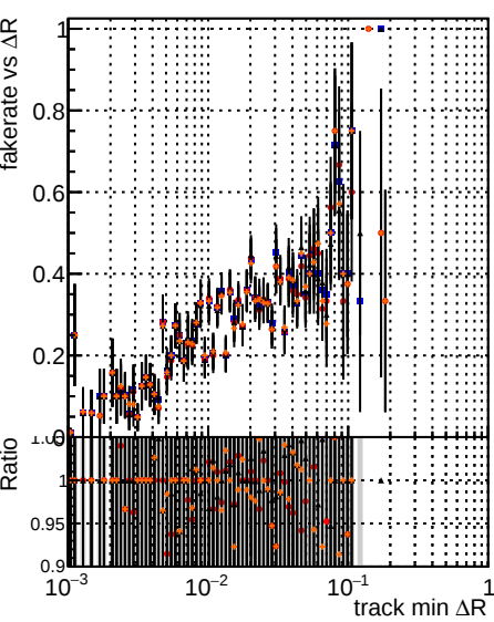
Fake rate vs \Delta R(\text{track, jet}) DOM mkt fit T-base retrainOldFiles125_v2_prelimWP_5iter retrainOldFiles125_v2_prelimWP_6iter retrainV2_WP2_6iter
