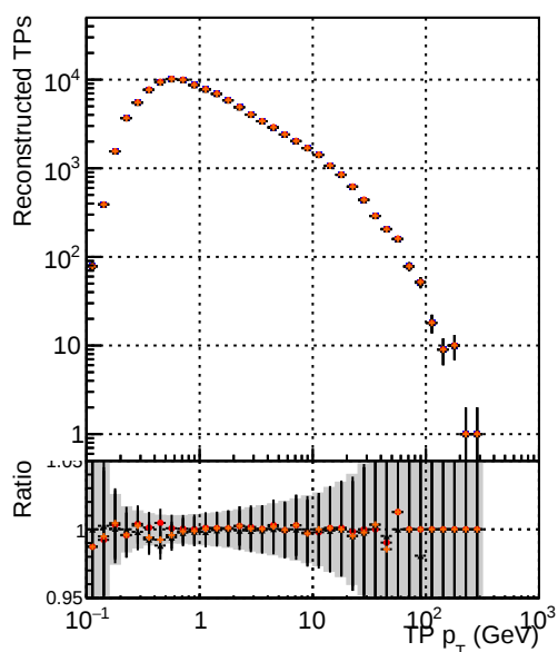
N of associated tracks (simToReco) vs TP p_T
