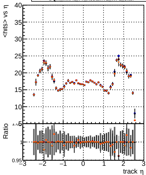
mean hits DOM_mkFit_TTbase DOM_mkFit_TT_retrainOldFiles125_v2_prelimWP_5iter DOM_mkFit_TT_baseline_6iter DOM_mkFit_TT_RetrainV2_WP2_6iter
