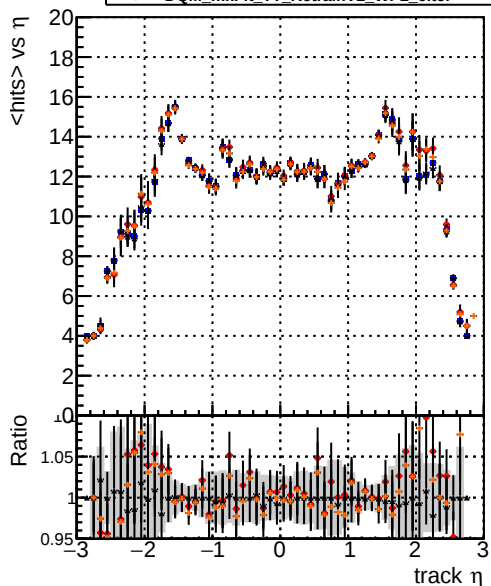
mean hits vs \eta Legend: - DQM_mkFit_TTbase (blue line) - DQM_mkFit_TT_retrainOldFiles125_v2_prelimWP_5iter (red line) - DQM_mkFit_TT_baseline_6iter (black line) - DQM_mkFit_TT_RetrainV2_WP2_6iter (orange line)
