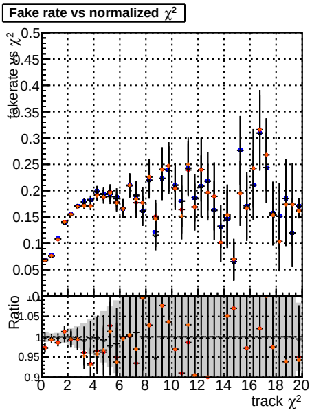
Fake rate vs. - Blue circles: DQM mkFit TTbase - Orange stars: DataTrainOldFiles125 v2 prelimWP_5iter - Red stars: DataTrainV2 WP2 6iter
