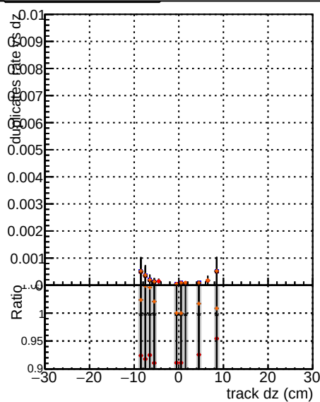
Legend: DOM mkFit TTbase, Data OldFiles125 v2 prelimWP_5iter, DOM mkFit RetrainV2 WP2 6iter
