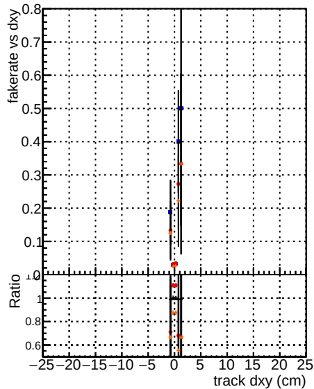
Legend: DOM mkFit TTbase, Data OldFiles125 v2 prelimWP_5iter, DOM mkFit RetrainV2 WP2 6iter
