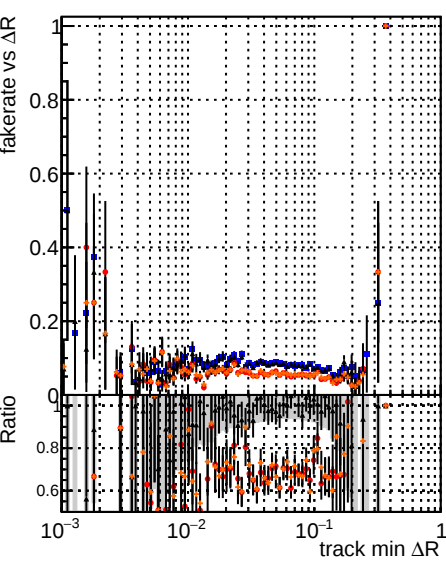
Fake rate vs \Delta R(\text{track, jet}) DOM mkt fit Tbase retrainOldFiles125_v2_prelimWP_5iter Baseline 6iter RetrainV2 WP2 6iter
