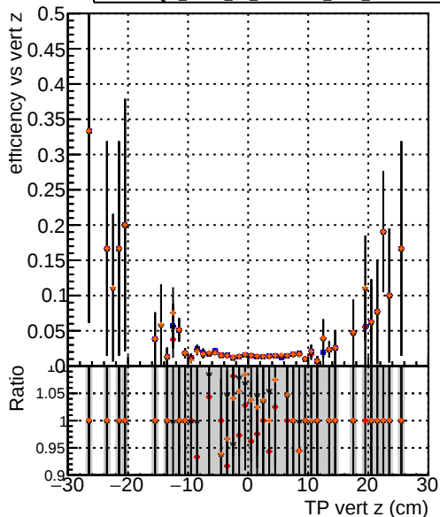
Efficiency vs. TP vert z (cm) Legend: - DQM_mkFit_TTbase (blue circles) - DQM_mkFit_TT_retrainOldFiles125_v2_prelimWP_5iter (red stars) - DQM_mkFit_TT_baseline_6iter (black triangles) - DQM_mkFit_TT_RetrainV2_WP2_6iter (orange crosses)
