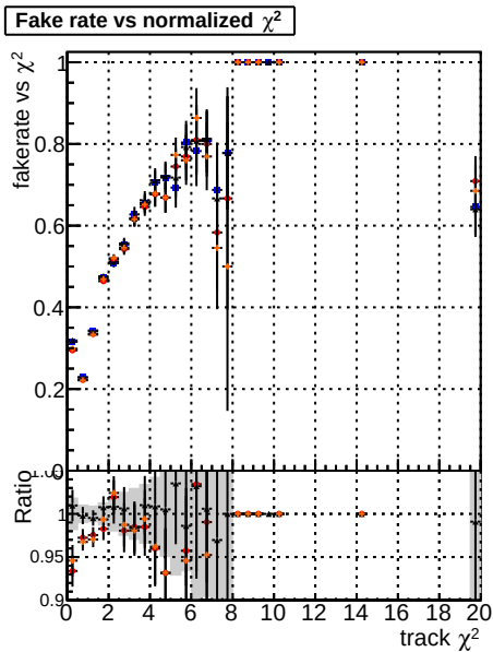
Fake rate vs. Legend: DGM mkFit, Tbase, RetrainOldFiles125 v2 prelimWP_5iter, RetrainV2 WP2 6iter
