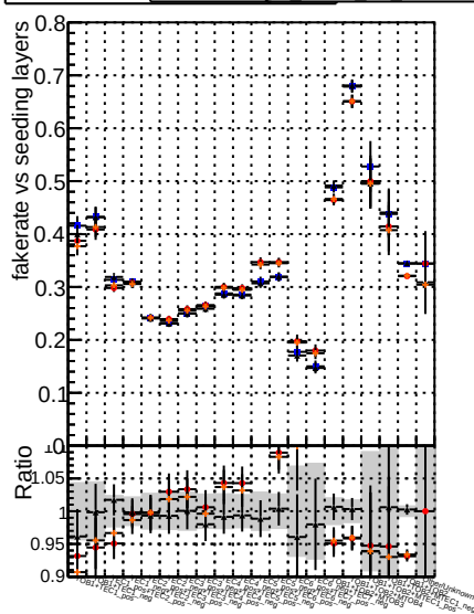
Fake rate vs. Legend: DGM mkFit, Tbase, RetrainOldFiles125 v2 prelimWP_5iter, RetrainV2 WP2 6iter
