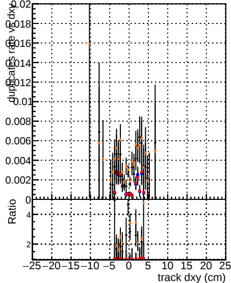
Legend for all plots: Blue circles: DQM mktFit Black circles: Tbase Orange circles: Retrain v2 WP2 Red circles: Retrain v2 WP2 6iter
