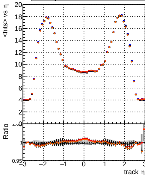
Legend: DQM_mkFit_TTbase (blue line), DQM_mkFit_TT_retrainOldFiles125_v2_prelimWP_5iter (red line with dots), DQM_mkFit_TT_baseline_6iter (black line with dots), DQM_mkFit_TT_RetrainV2_WP2_6iter (orange line with dots) mean hit
