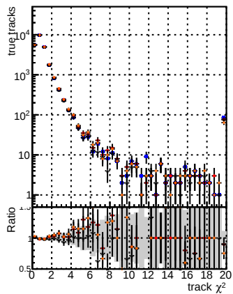
N of reco track vs. \chi^2 BSM mktFit TTbase BSM mktFit TTbase+oldFiles125_v2_prelimWP_5iter BSM mktFit TTbase+oldFiles125_v2_prelimWP_5iter+RefrainV2_WP2_6iter
