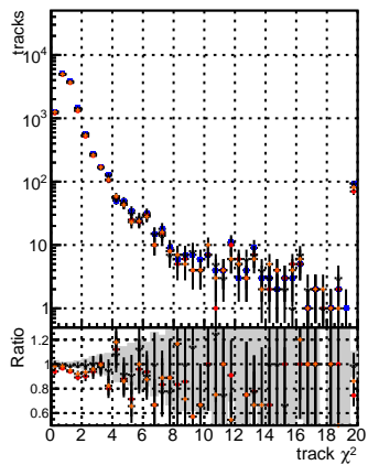
N of reco track vs. \chi^2 for BGM mFit TTbase Retrain v2 WP2 6iter Retrain Old Files125_v2_prelimWP_5iter
