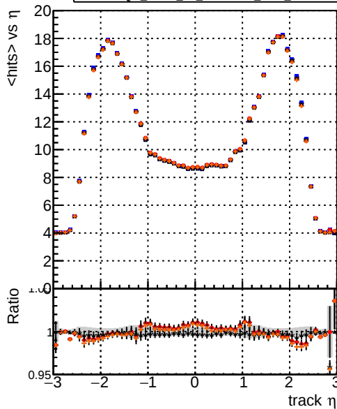
mean hit DOM_mkFit_TTbase DOM_mkFit_TT_retrainOldFiles125_v2_prelimWP_5iter DOM_mkFit_TT_baseline_6iter DOM_mkFit_TT_RetrainV2_WP2_6iter
