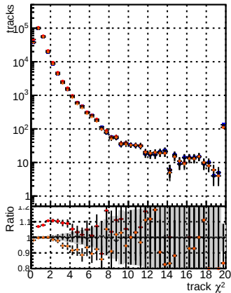
N of reco track vs. s DOM mkt-fit T-base RetrainOldFiles125_v2_prelimWP_5iter Baseline --- --- --- --- RetrainV2_WP2_6iter --- --- --- ---
