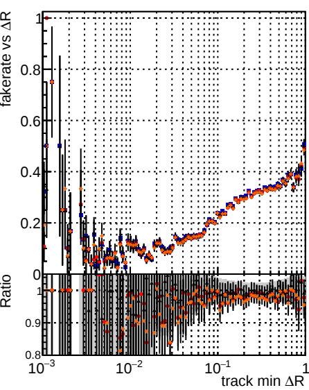
Fake rate vs \Delta R (track, jet) Legend: DOM mkFit TTbase, DOM mkFit TTbase, RetrainOldFiles125_v2_prelimWP_5iter, RetrainOldFiles125_v2_prelimWP_5iter, RetrainV2_WP2_6iter, RetrainV2_WP2_6iter
