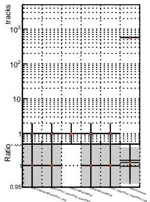
N of reco track vs. \chi^2 BGM mFit \chi^2 base BGM mFit \chi^2 base + 125 v2 prelim WP 5iter BGM mFit \chi^2 base + 125 v2 prelim WP 6iter
