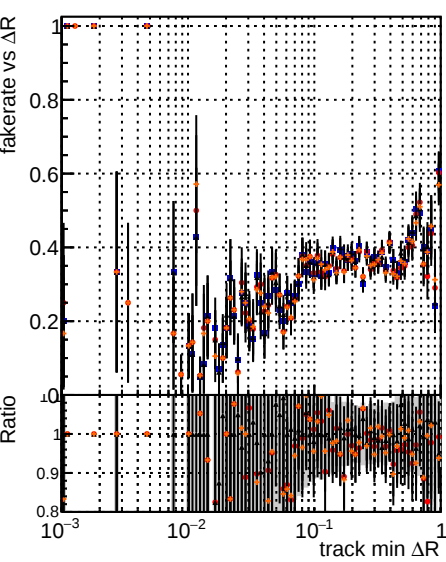
Fake rate vs \Delta R(\text{track, jet}) Legend: DOM (black) mkFit (blue) T-base (red) retrainOldFiles125_v2_prelimWP_5iter (orange) RetrainOldFiles125_v2_prelimWP_6iter (green) RetrainV2_WP2_6iter (purple) RetrainV2_WP2_5iter (brown)
