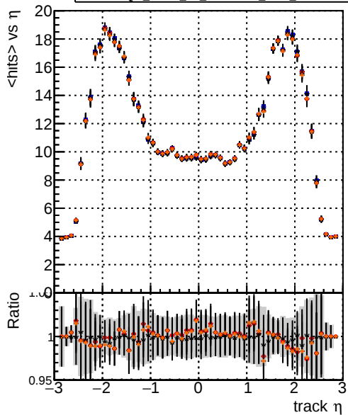
mean hits Legend: DQM_mkFit_TTbase (blue line) DQM_mkFit_TT_retrainOldFiles125_v2_prelimWP_5iter (red line with error bars) DQM_mkFit_TT_baseline_6iter (black line with error bars) DQM_mkFit_TT_RetrainV2_WP2_6iter (orange line with error bars)
