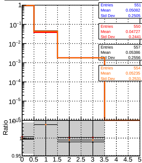
mean hit Legend: - DQM_mkFit_TTbase (blue line with circles) - DQM_mkFit_TT_retrainOldFiles125_v2_prelimWP_5iter (red line with circles) - DQM_mkFit_TT_baseline_6iter (black line with circles) - DQM_mkFit_TT_RetrainV2_WP2_6iter (orange line with circles)
