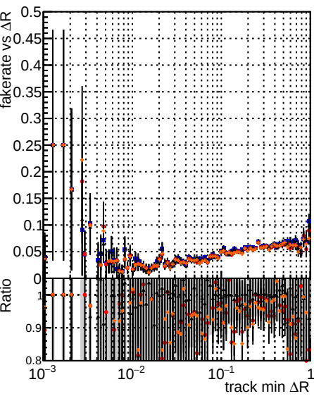
Fake rate vs \Delta R(\text{track, jet}) Legend: DOM mkFit TTbase DOM mkFit TTbase RetrainOldFiles125_v2_prelimWP_5iter DOM mkFit TTbase RetrainOldFiles125_v2_prelimWP_5iter RetrainV2_WP2_6iter
