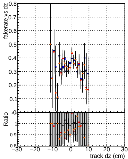
Fake rate vs d Legend: DOM (blue square), mkFit (red circle), TTbase (green triangle), RetrainOldFiles125_v2_prelimWP_5iter (orange diamond), RetrainOldFiles125_v2_prelimWP_6iter (purple star), Retrainv2_WP2_6iter (brown cross). Models: DOM, mkFit, TTbase, RetrainOldFiles125_v2_prelimWP_5iter, RetrainOldFiles125_v2_prelimWP_6iter, Retrainv2_WP2_6iter.
