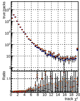
N of reco track vs. \chi^2 for BSM m1E11, BSM m1E12, BSM m1E13, BSM m1E14, BSM m1E15, BSM m1E16, BSM m1E17, BSM m1E18, BSM m1E19, BSM m1E20, BSM m1E21, BSM m1E22, BSM m1E23, BSM m1E24, BSM m1E25, BSM m1E26, BSM m1E27, BSM m1E28, BSM m1E29, BSM m1E30, BSM m1E31, BSM m1E32, BSM m1E33, BSM m1E34, BSM m1E35, BSM m1E36, BSM m1E37, BSM m1E38, BSM m1E39, BSM m1E40, BSM m1E41, BSM m1E42, BSM m1E43, BSM m1E44, BSM m1E45, BSM m1E46, BSM m1E47, BSM m1E48, BSM m1E49, BSM m1E50, BSM m1E51, BSM m1E52, BSM m1E53, BSM m1E54, BSM m1E55, BSM m1E56, BSM m1E57, BSM m1E58, BSM m1E59, BSM m1E60, BSM m1E61, BSM m1E62, BSM m1E63, BSM m1E64, BSM m1E65, BSM m1E66, BSM m1E67, BSM m1E68, BSM m1E69, BSM m1E70, BSM m1E71, BSM m1E72, BSM m1E73, BSM m1E74, BSM m1E75, BSM m1E76, BSM m1E77, BSM m1E78, BSM m1E79, BSM m1E80, BSM m1E81, BSM m1E82, BSM m1E83, BSM m1E84, BSM m1E85, BSM m1E86, BSM m1E87, BSM m1E88, BSM m1E89, BSM m1E90, BSM m1E91, BSM m1E92, BSM m1E93, BSM m1E94, BSM m1E95, BSM m1E96, BSM m1E97, BSM m1E98, BSM m1E99, BSM m1E100.
