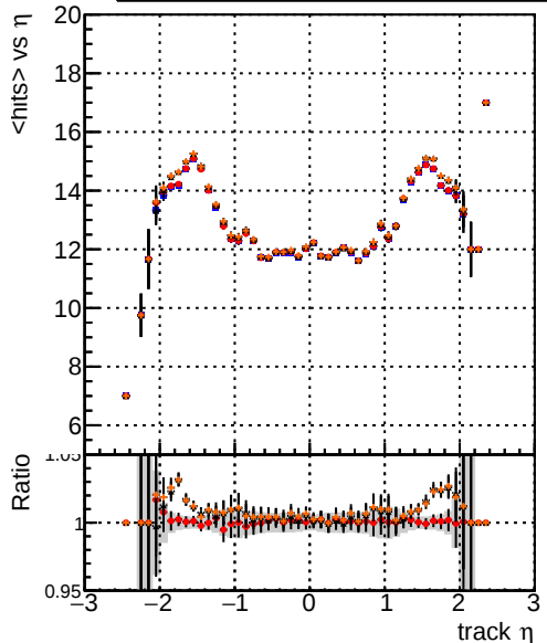
mean hits vs \eta DOM_mkFit_TTbase DOM_mkFit_TT_retrainOldFiles125_v2_prelimWP_5iter DOM_mkFit_TT_baseline_6iter DOM_mkFit_TT_RetrainV2_WP2_6iter
