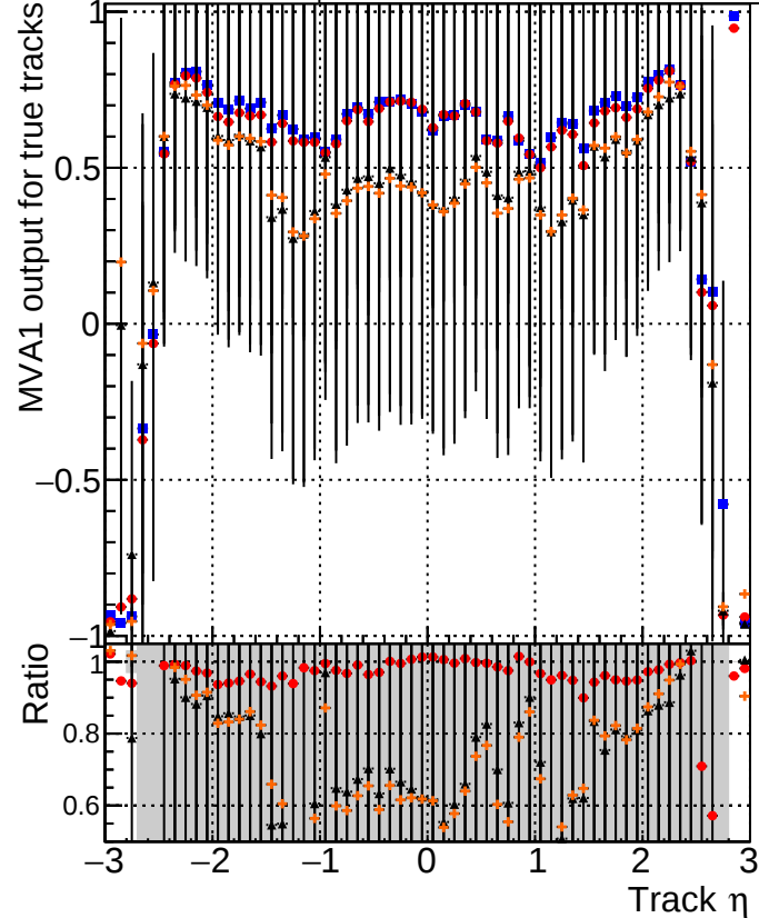
MVA1 of associated tracks (recoToSim) vs. track \eta Legend: DQM_mkFit_TTbase (blue squares) DQM_mkFit_TT_retrainOldFiles125_v2_prelimWP_5iter (red diamonds) DQM_mkFit_TT_baseline_6iter (black stars) DQM_mkFit_TT_RetrainV2_WP2_6iter (orange stars)
