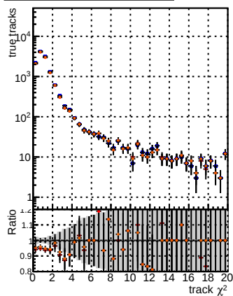
N of reco track vs. \chi^2 for BSM mktFit + Base, BSM mktFit + Retrain Old Files, BSM mktFit + Retrain V2 WP2 5iter
