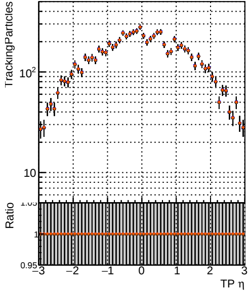
N of simulated tracks vs \eta Legend: DOM_mkFit_TTbase DOM_mkFit_TT_retrainOldFiles125_v2_prelimWP_5iter DOM_mkFit_TT_baseline_6iter DOM_mkFit_TT_RetrainV2_WP2_6iter
