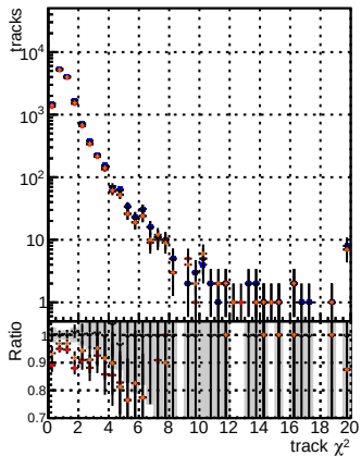
N of reco track vs. s DOM mkefit TT base RetrainOldFiles125_v2_prelimWP_5iter baseLine 6iter DOM mkefit TT base RetrainV2 WP2 6iter
