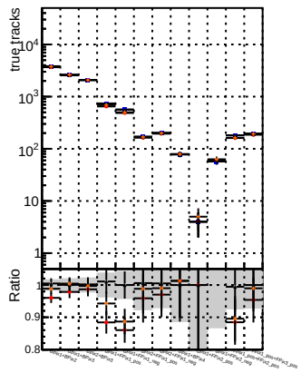
N of reco track vs. s DOM mkefit TT base RetrainOldFiles125_v2_prelimWP_5iter baseLine 6iter DOM mkefit TT base RetrainV2 WP2 6iter
