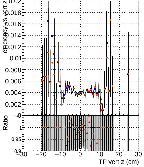
Efficiency vs. TP vert z DOM_mkFit_TTbase DOM_mkFit_TT_retrainOldFiles125_v2_prelimWP_5iter DOM_mkFit_TT_baseline_6iter DOM_mkFit_TT_RetrainV2_WP2_6iter
