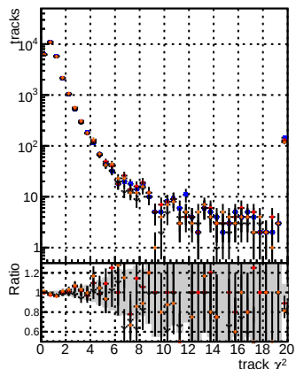
N of reco track vs. \chi^2 for BSM mktFit TTbase, BSM mktFit TTbase+oldFiles125_v2_prelimWP_5iter, and BSM mktFit TTbase+oldFiles125_v2_prelimWP_5iter+RefrainV2_WP2_6iter
