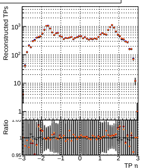
N of associated tracks (simToReco) vs TP \eta
