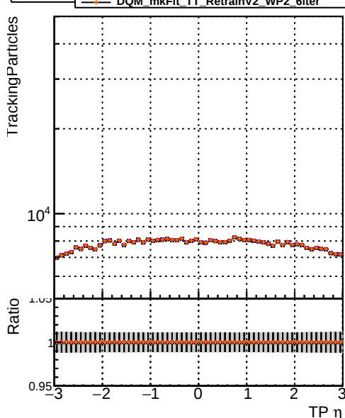
N of simulated tracks vs TP \eta
