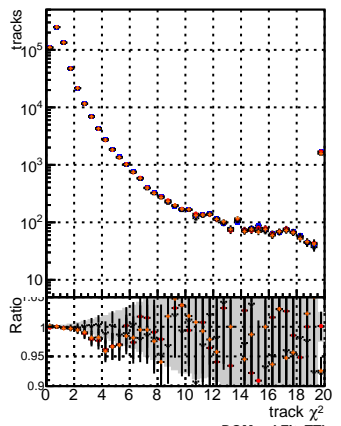
N of reco track vs. \chi^2 for various algorithms: BGM, mFit, Refrain, OldFiles, 125_v2_prelimWP_5iter, RefrainV2, WP2_6iter
