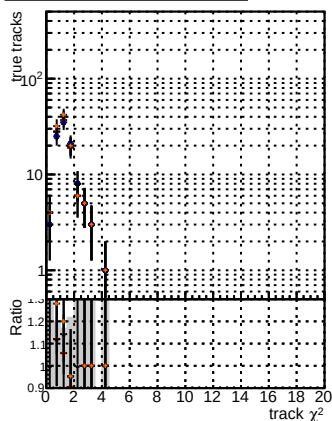
N of reco track vs. \chi^2 for various models: BSM mxFit (blue), BSM mxFit + base (orange), BSM mxFit + base + 125 v2 prelim (black), BSM mxFit + base + 125 v2 prelim + 5iter (grey), and BSM mxFit + base + 125 v2 prelim + 5iter + 6iter (red).
