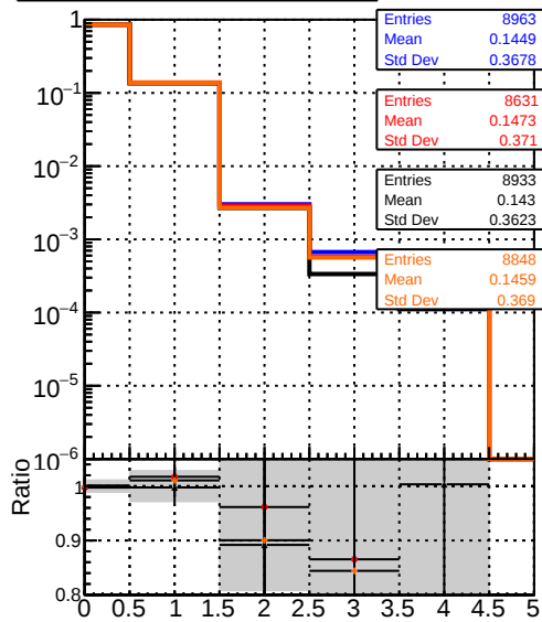
mean hit DOM_mkFit_TTbase DOM_mkFit_TT_retrainOldFiles125_v2_prelimWP_5iter DOM_mkFit_TT_baseline_6iter DOM_mkFit_TT_RetrainV2_WP2_6iter
