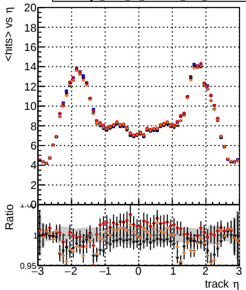
mean hits vs \eta Legend: - DQM_mkFit_TTbase (blue line) - DQM_mkFit_TT_retrainOldFiles125_v2_prelimWP_5iter (red line with error bars) - DQM_mkFit_TT_baseline_6iter (black line with error bars) - DQM_mkFit_TT_RetrainV2_WP2_6iter (orange line with error bars)
