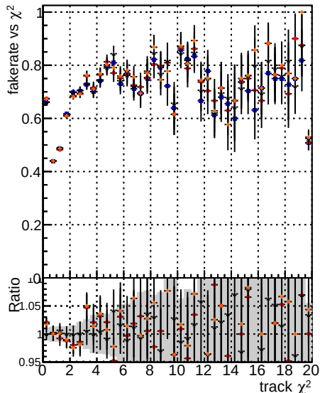
Fake rate vs. Legend: BQM mkFit TTbase BQM mkFit RetrainV2 WP2 6iter
