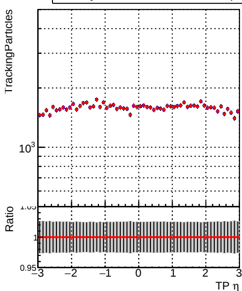
N of simulated tracks vs \eta Legend: \blacksquare DQM_mkFit_TTbase \bullet DQM_mkFit_TT_retrainOldFiles125_v2_prelimWP_5iter
