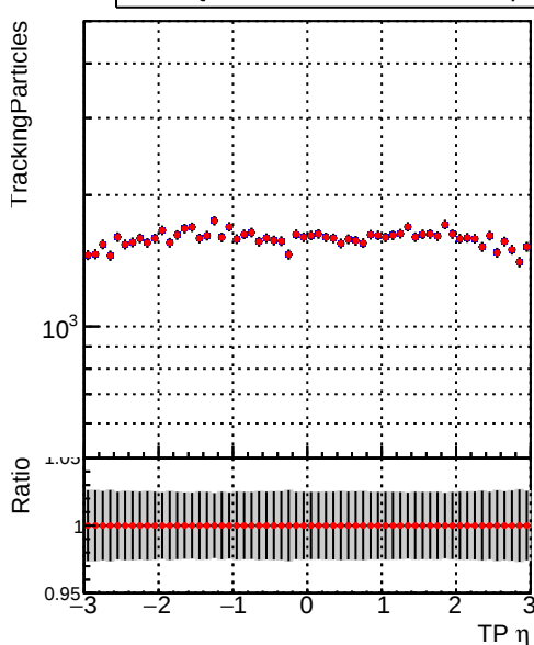
N of simulated tracks vs TP \eta — DQM_mkFit_TTbase — DQM_mkFit_TT_retrainOldFiles125_v2_prelimWP_5iter
