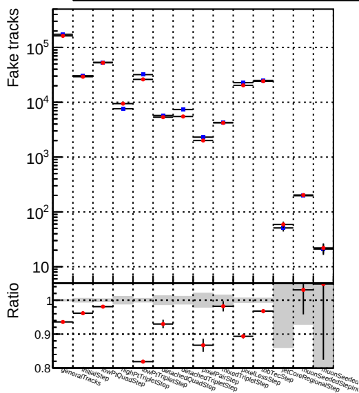
Number File 1 DQM_mkFit_TT_retrainOldFiles125_v2_prelimWP_5iter
