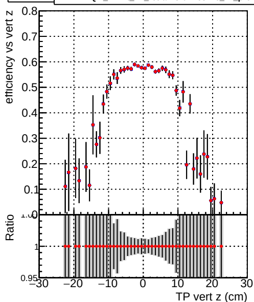
Efficiency vs. sim PV z —●— DQM_mkFit_TTbase —●— DQM_mkFit_TT_retrainOldFiles125_v2_prelimWP_5iter
